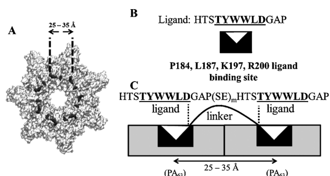
Scheme 2. Representation of binding of the polypeptide-based inhibitors to adjacent sites on (PA_{63})_7 . A) Structure of (PA_{63})_7 with black dots on individual PA_{63} monomers representing the predicted binding sites (P184, L187, K197, and R200) for the 12-mer ligand. B) Representation showing the interaction of the 6-mer TYWWLD (white triangle) with its binding site on PA_{63} (black sector symbol). C) Representation of interactions between a divalent polypeptide and binding sites on adjacent PA_{63} monomers of (PA_{63})_7 .
